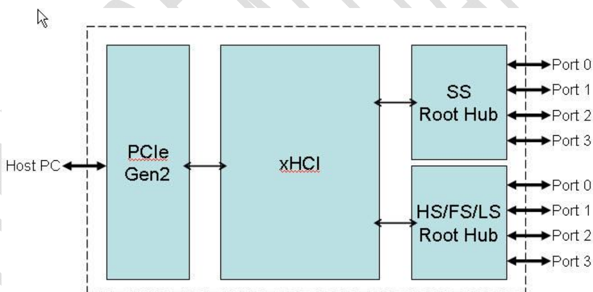
Figure 1: EJ188 Block Diagram
